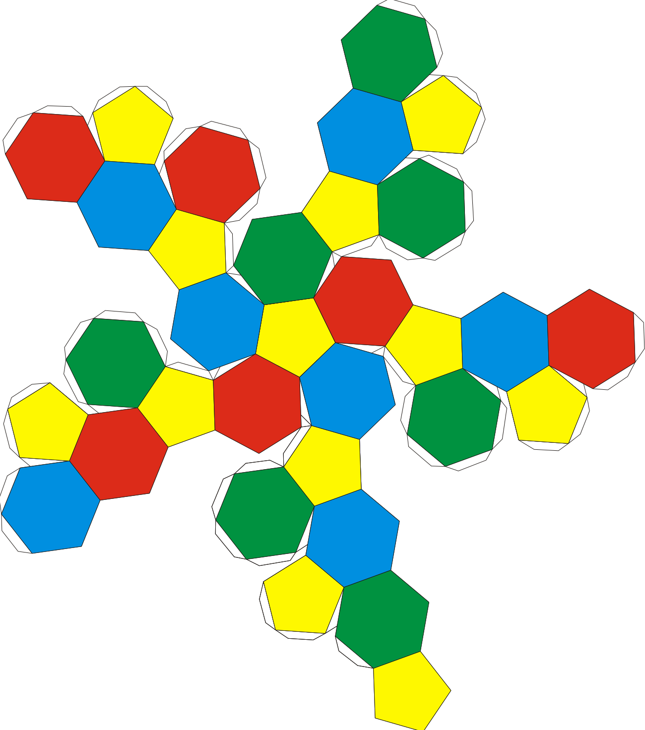
Truncated Icosahedron
