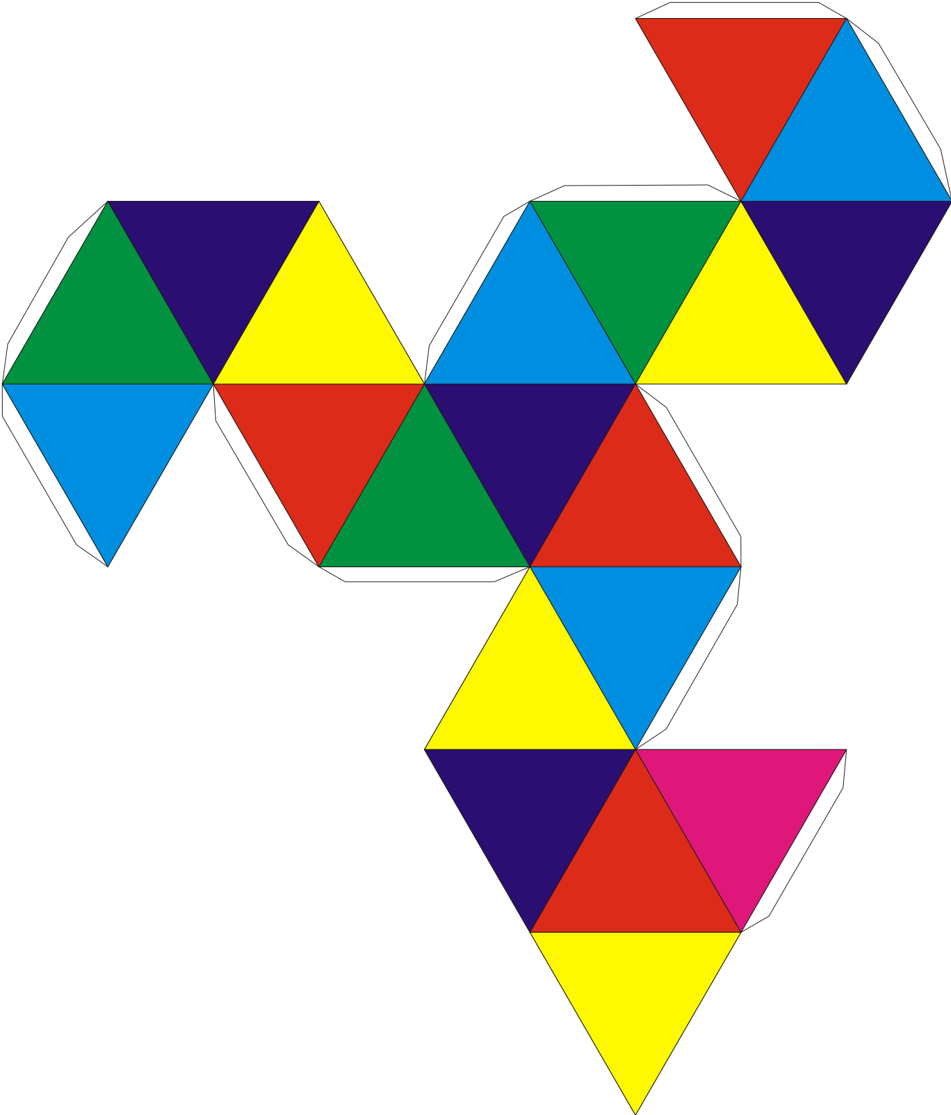
Icosahedron
